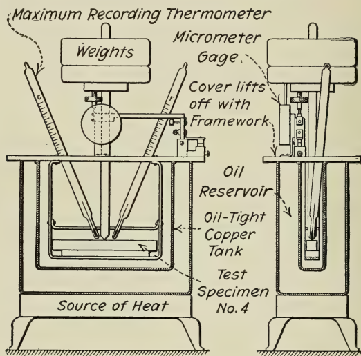
FIG. 194.—Apparatus for Recording Distortion of Bituminized Aggregates under Heat.
